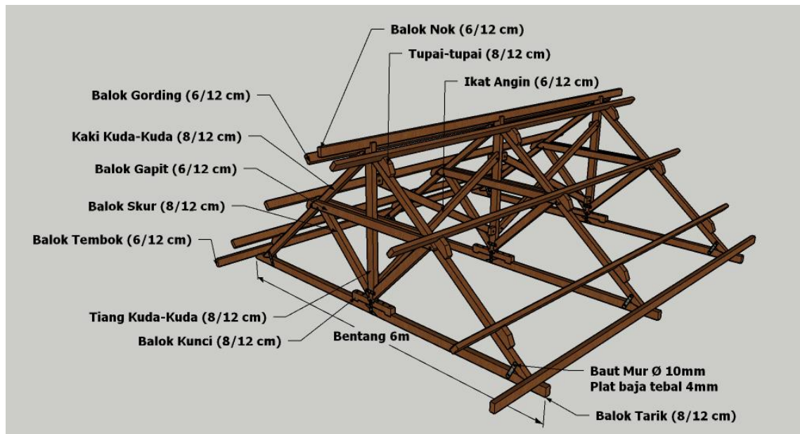
Figure 2. Three-dimensional roof-truss visualization developed in SketchUp
