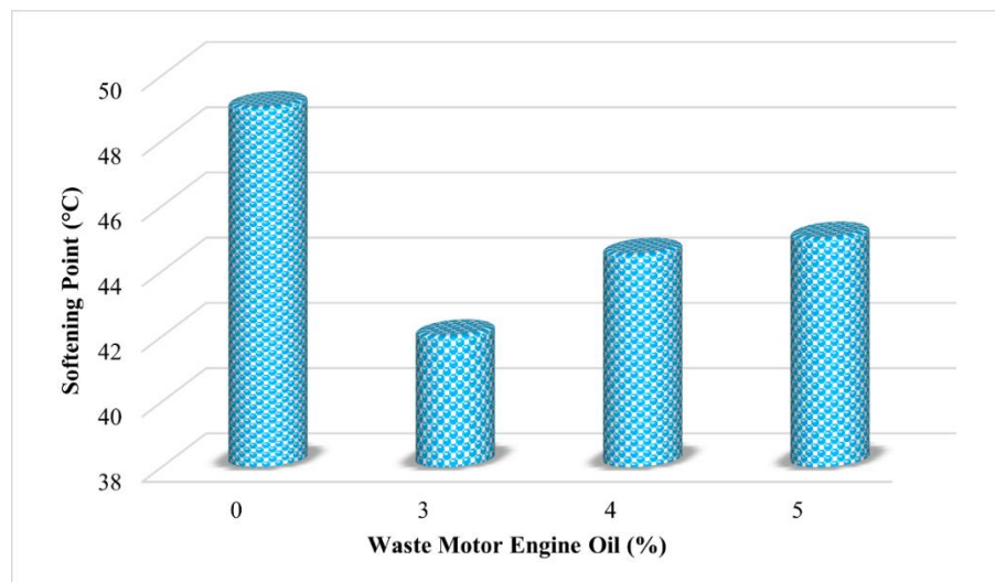
Figure 2: Softening point value of waste motor engine oil in warm mix asphalt
