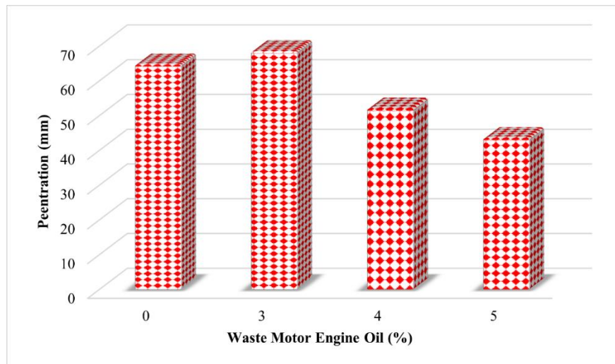
Figure 1: Penetration value of waste motor engine oil in warm mix asphalt
