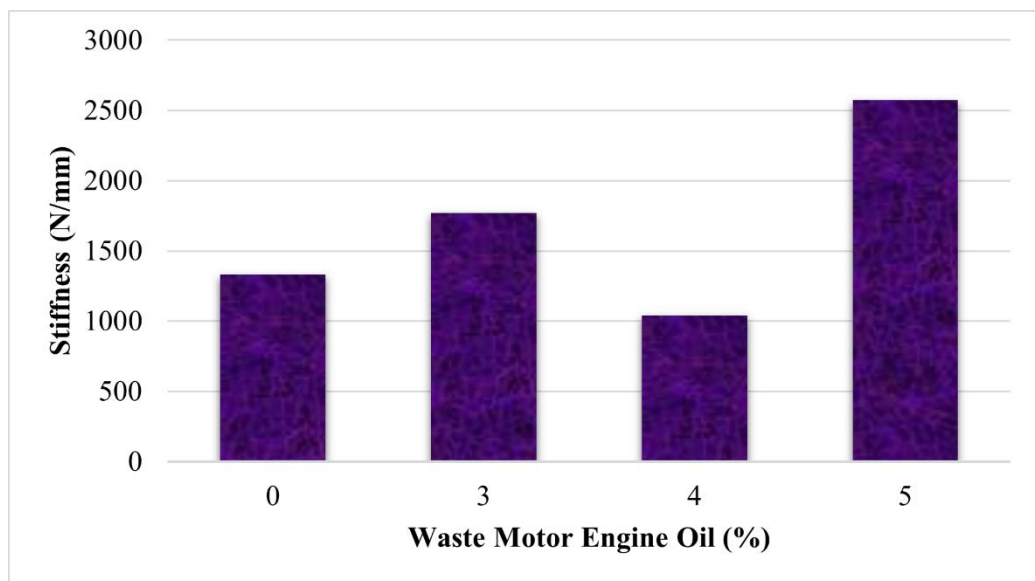
Figure 5: Stiffness of warm mix asphalt containing waste motor engine oil
