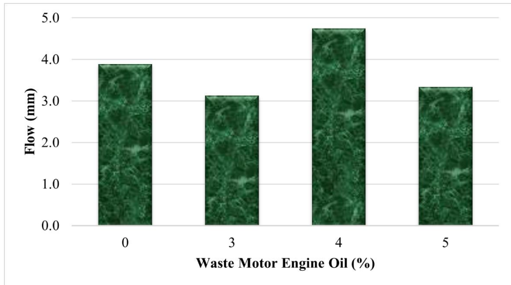
Figure 4: Flow of warm mix asphalt containing waste motor engine oil
