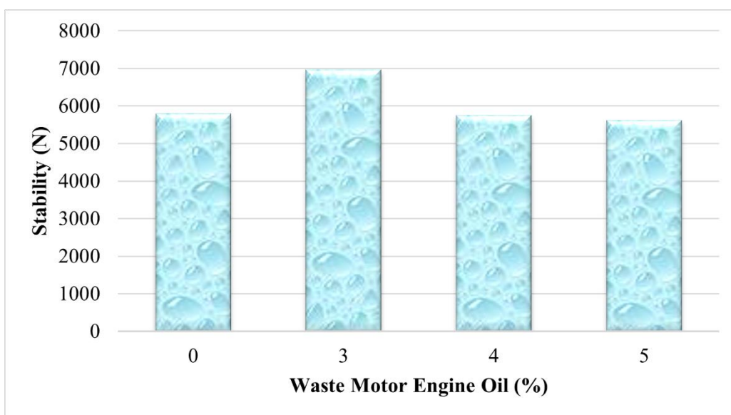
Figure 3: Stability of warm mix asphalt containing waste motor engine oil.
