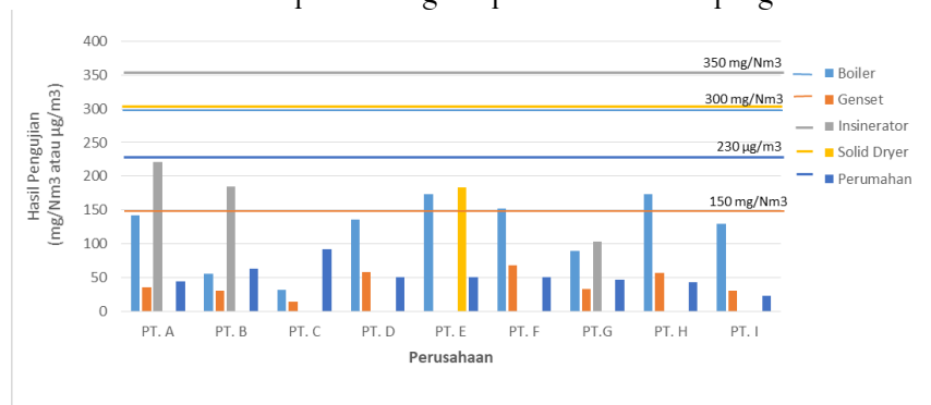
Figure 2. Comparison of the results of particulate testing with TSP (Dust)
