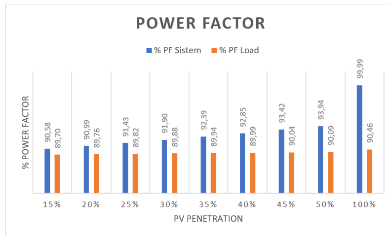
Figure 5. 80% Inverter power factor
