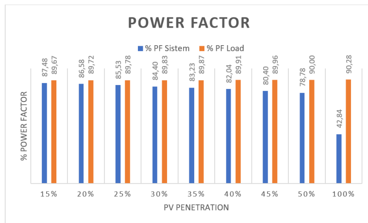
Figure 3. 100% Inverter power factor
