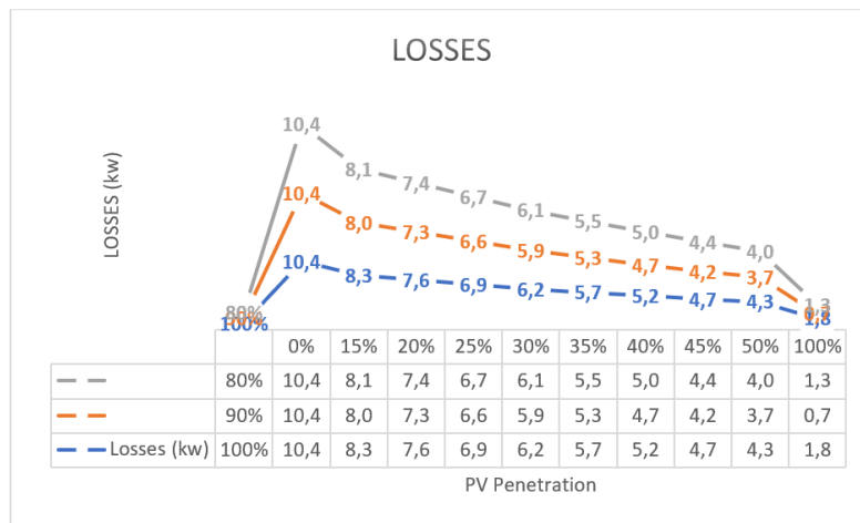
Figure 6. System Losses for different Power Factor
