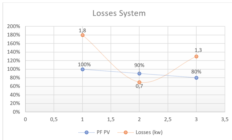
Figure 7. U-Shape Power Factor's Curve
