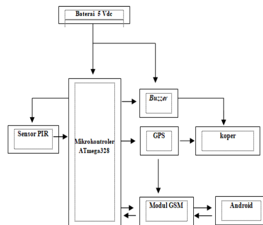
Figure 7. Diagram Block
