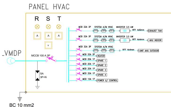
Figure 1. Single Line Diagram of HVAC Panel
