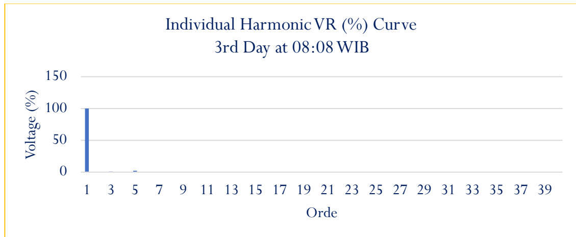
Figure 3. Individual Voltage R Harmonic (%) Measurement Curve on 3 rd at 08:08 WIB
