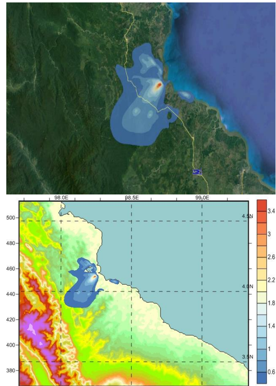
Figure 5. Simulation Results of SO 2 Distribution Patterns (Total Period Average) around PLTU Pangkalan Susu
