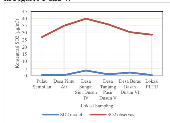
Figure 3. SO 2 Model Concentration and Observation SO 2 Concentration at PLTU Pangkalan Susu
